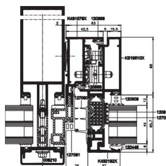
One of the most important advantages of this solution are the unusually economical shapes, which add lightness to the entire structure. Thanks to application of the most modern technology of structural gluing, based on gluing the outer glass panel to the aluminium frame with structural silicon, we have avoided the necessity to use any aluminium elements from the outside or any mechanical joints for fitting the glass panel.
