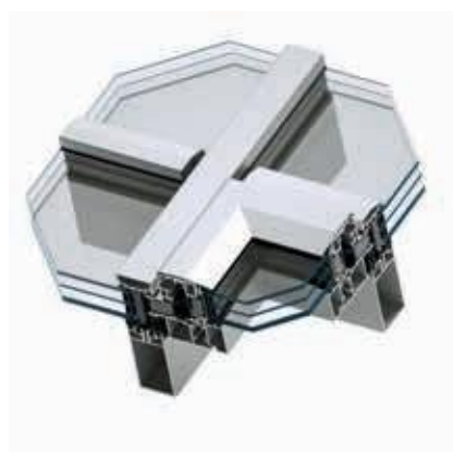
Windows fabricated using the MB-RW system are intended for installation on roofs with mullion-transom systems (MB-SR50N & MB-TT50 group of products) of an inclination angle of 3° to 75° in relation to the horizontal plane. In rafters/purlins axes, roof windows can have dimensions up to 2.5 m and weight up to 200 kg.
