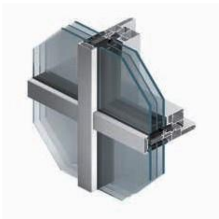
MB-SR50N IW enables the use of inward openable windows integrated with mullion-transom profiles. The area of the façade with tilt-andturn function does not differ, as seen from the outside, from the neighbouring areas with fixed glazing. This systems comes in 3 varieties: standard, with flat strip and EFEKT.
